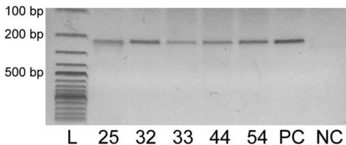
Figure 1. Agarose gel electrophoresis of QPCR amplicon 225 bp SEC amplicons, lane L- 100 bp ladder, lane 25; 32; 33; 44; 54 – isolates, lane PC-ATCC 19095 S. aureus SEC positive, lane NC-negative control
