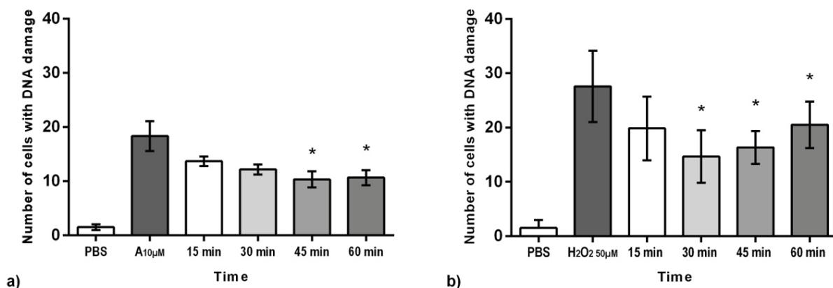
Figure 2 DNA damage repair in cells exposed to a) adrenaline (A) and b) H 2 O 2 at 15, 30, 45, and 60 min after treatment. Bars represent the mean number of cells with DNA damage (B+C+D+E comet classes) ±SEM; * p<0.05 vs. adrenaline- and H 2 O 2 -treated control
