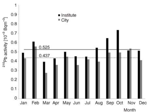
Figure 4. Monthly means of ^{210}\text{Pb} activities (the key as in fig. 3)
