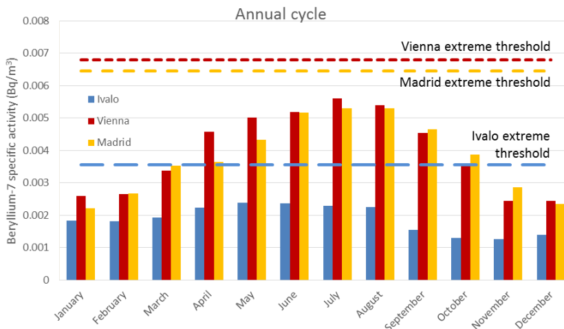
Fig. 2 Monthly mean Be-7 specific activities over the 2001–2010 period (bars) and extreme thresholds (95 th percentile) (dashed lines) for Ivalo (blue), Vienna (red) and Madrid (yellow).
