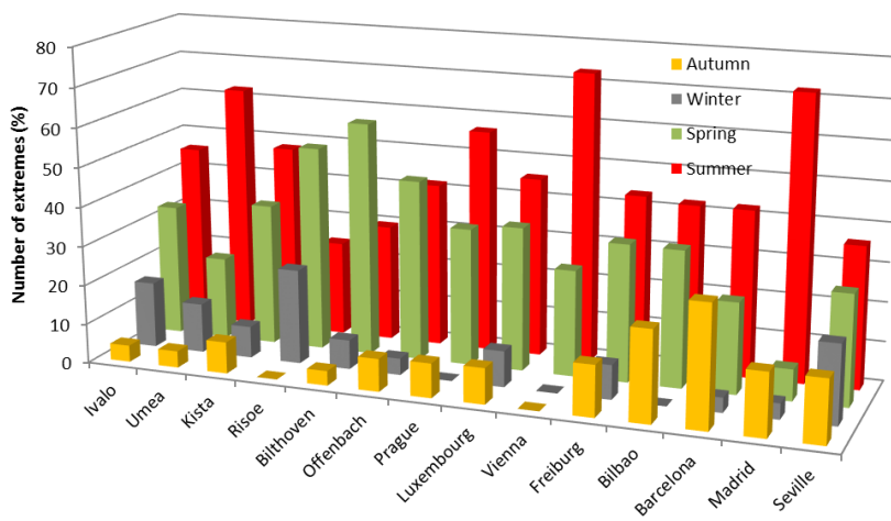
Fig. 3 Number of extremes in the Be-7 specific activity (as percent of the total number of extremes) per season.
