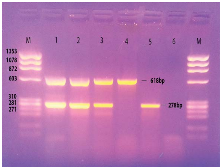
Figure 3. Agarose gel electrophoresis with PCR products obtained in multiplex PCR for Pseudomonas and Stenotrophomonas (for 3 unidentified strains): lane M-ΦX174 DNA/BsuRI (HaeIII) Marker, 9 (Fermentas); lanes 1-3 strains positive on both genera with 618 and 278 bp PCR products; lane 4 P.aeruginosa ATCC 27853; lane 5 S. maltophilia ATCC 13637; lane 6 negative control for PCR.
