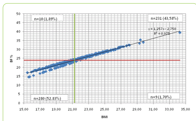
Figure 2: Correlation between body mass index (BMI) and percent body fat (% BF) for 530 girls 15 to 19 years old.
