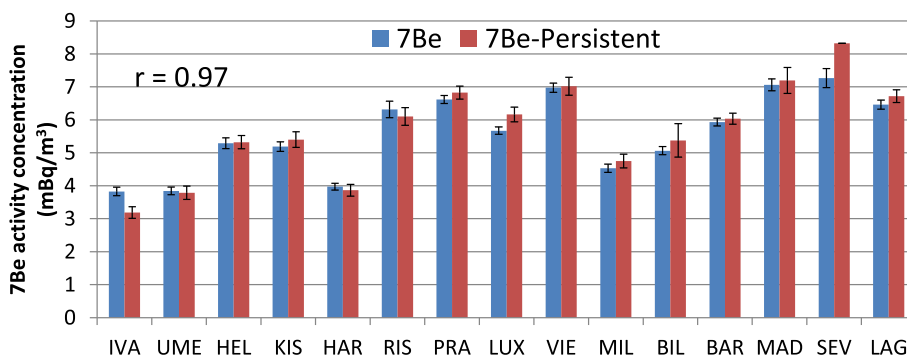
Fig. 6. Comparison of the mean 7 Be activity concentration of all the measurements higher or equal P90 (peak 7 Be) (blue bar) and the mean of the measurements higher or equal P90 only during the persistent periods (peak 7 Be-persistent) (red bar). (For interpretation of the references to colour in this figure legend, the reader is referred to the Web version of this article.)
