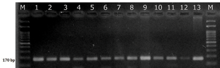
Figure 1. M – ladder; 1 – positive control for Red deer; 2 – hair (Red deer); 3 – positive control for Fallow deer; 4 – hair (Fallow deer); 5 – positive control for Roe deer; 6 – hair (Roe deer); 7 - blood (Red deer); 8 – blood (Fallow deer); 9 – blood (Roe deer); 10 – pelt (Red deer); 11 – feces (Roe deer); 12 – feces (Fallow deer); 13 – spleen (Red deer)
